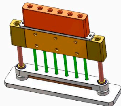
成型入芯一体模具 Forming core integrated mold
