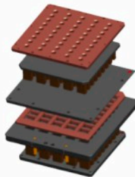
压粉模具 Pressed powder mold
