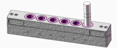
6孔倒灌口红模具 6-hole pour-over lipstick mold
