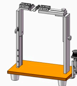
粉饼跌落测试台 Powder drop test bench
