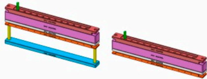
12孔双色口红模具 12 hole two-color lipstick mold
