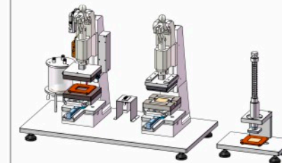
湿粉压粉机 Wet powder pressing machine
