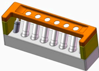
6孔正灌口红模具 6 hole filling lipstick mold
